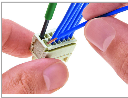
Inserting a conductor via (2.5 x 0.4) mm screwdriver – CAGE CLAMP® actuation parallel to conductor entry.
