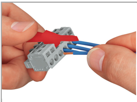
Conductor termination perpendicular to CAGE CLAMP® actuation
