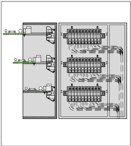
Multilevel arrangement in a distributed electronic housing
