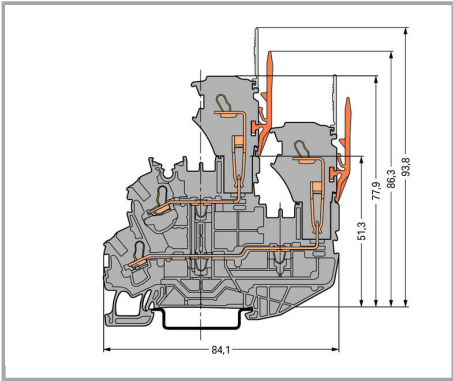
Double-deck carrier terminal block
