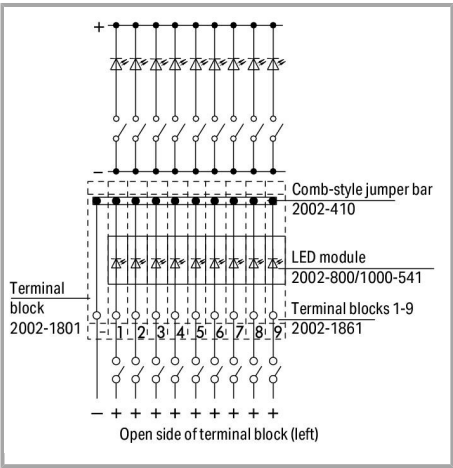
LED module (2002-800/1000-541)
