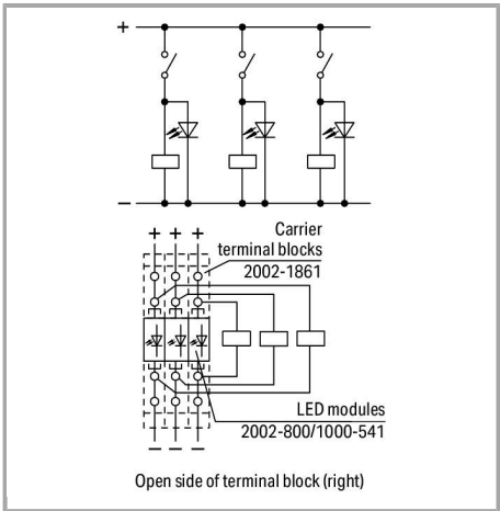
LED module (2002-800/1000-541)
