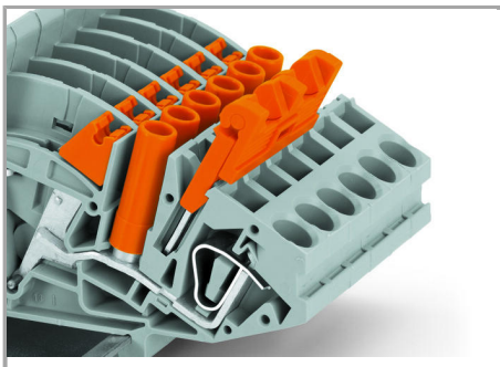
BJumper with safety lid in pre-locked position
