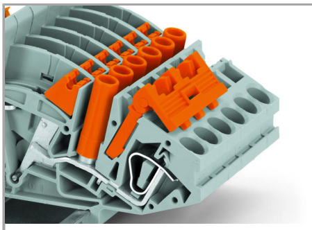
Longitudinal switching disconnect terminal blocks with inserted jumper, including safety lid
