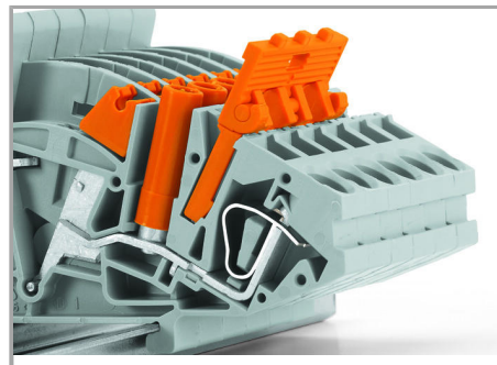
Jumper with raised safety lid
