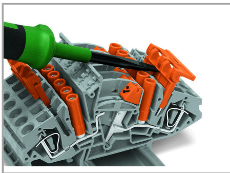
Jumper with safety lid:
