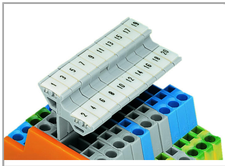
Labeling via WAGO Multi Marking System.
