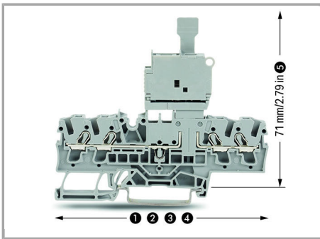
Fuse plug dimensions:
