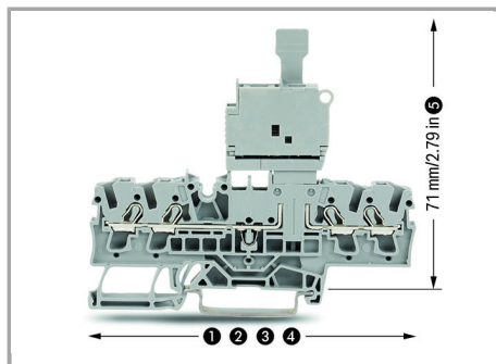
Fuse plug dimensions:
