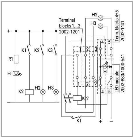
LED module (2002-880/1000-541)
