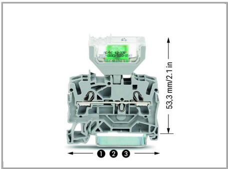
Dimensions of through terminal blocks with a pluggable LED module:
