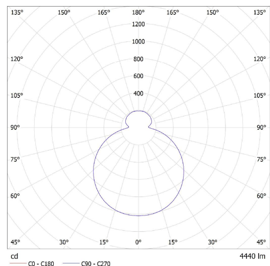
Lucis S46.K12.O60 FORUM LED / LDC (Polar)
